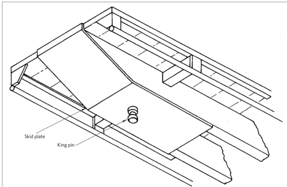
Figure 8-7-1. Kingpin and skid plate
