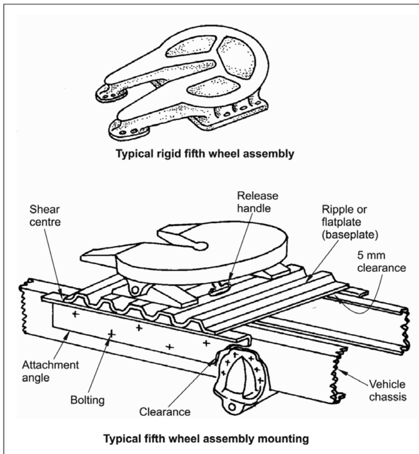
Figure 8-6-1. Fifth wheels
