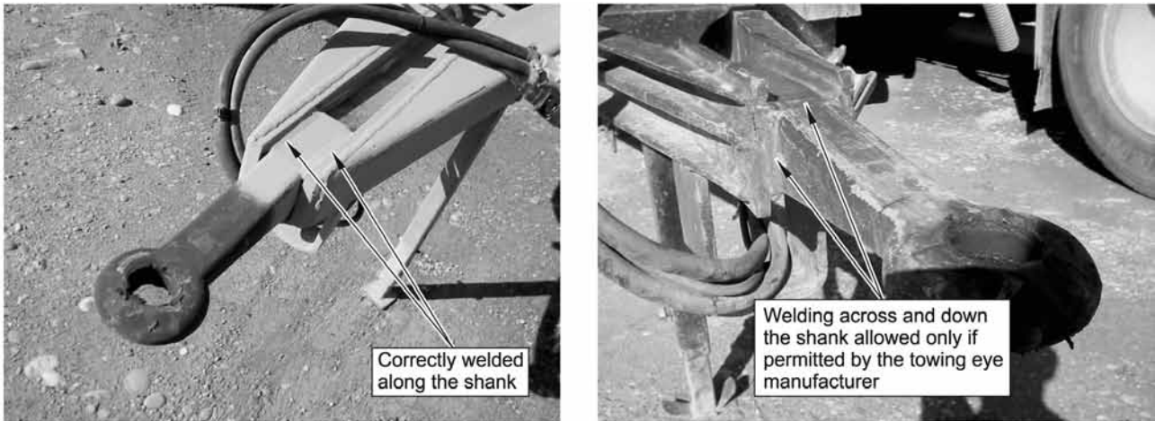
Figure 8-3-1. Permitted welding on towing eye shank
