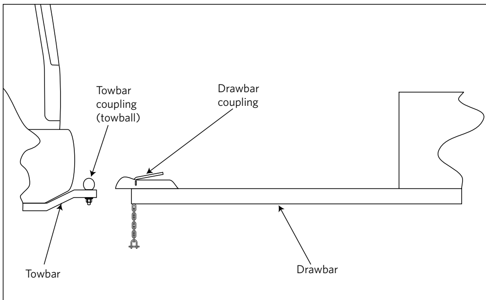
Figure 8-1-1. Tow coupling components
