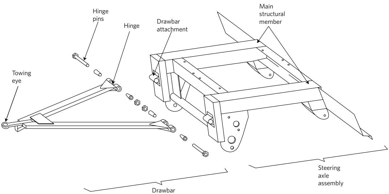
Figure 8-3-2. Drawbar components
