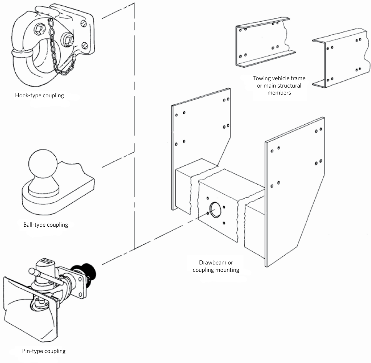
Figure 8-4-3. Drawbeam components
