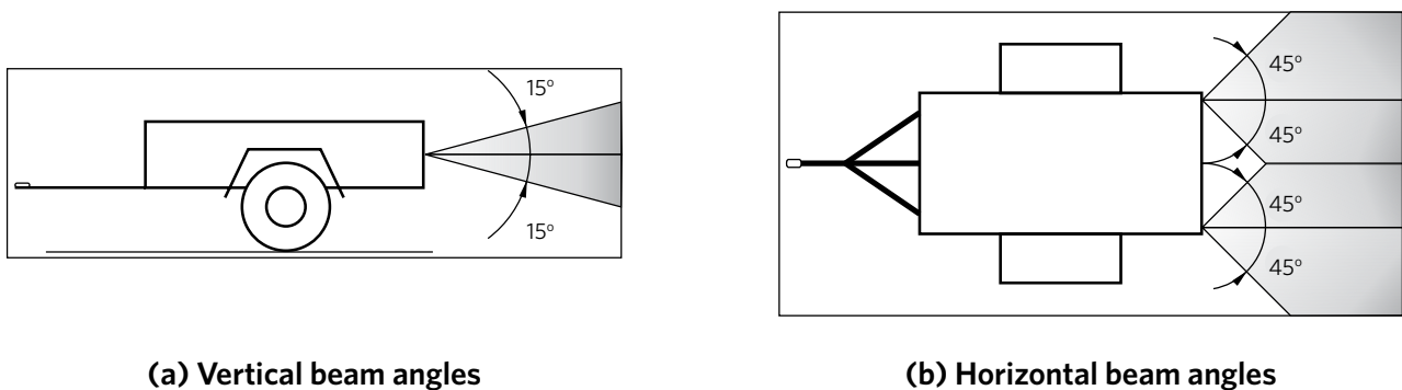
Figure 4-10-1. Stop lamp beam angles
