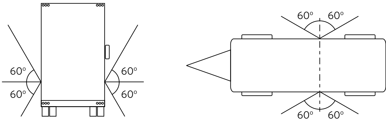
Figure 4-8-1. Visibility angles for side-marker lamps
