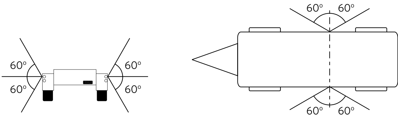
Figure 4-8-1. Visibility angles for side-marker lamps
