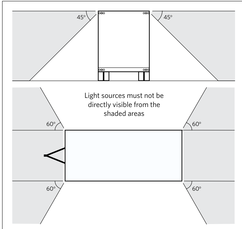
Figure 4-15-1. Visibility angles for cosmetic lamps
