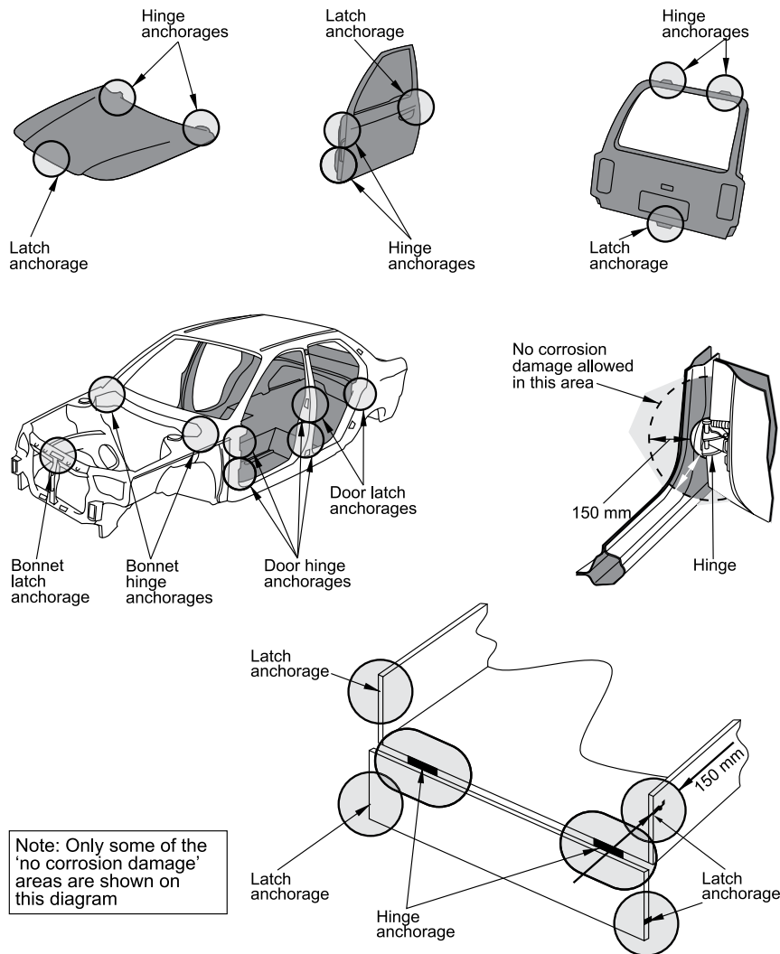
Figure 6-1-1. Hinge and latch anchorages
