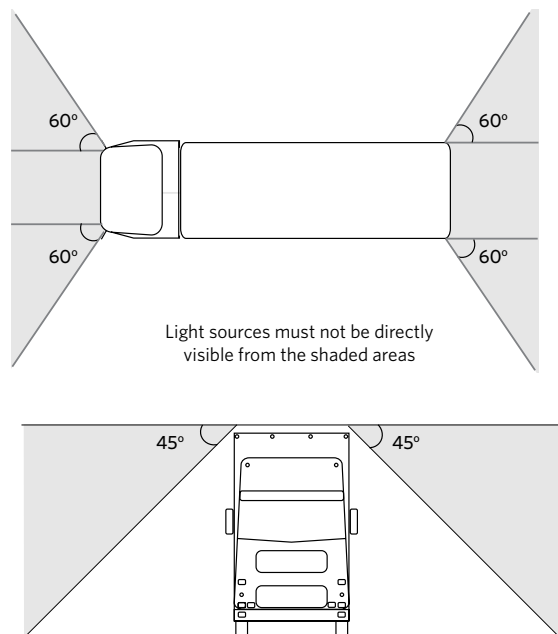
Figure 4-15-1. Visibility angles for cosmetic lamps
