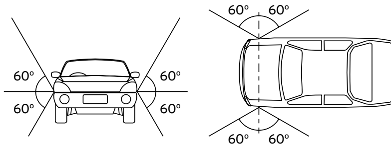
Figure 4-8-1. Visibility angles for side-marker lamps
