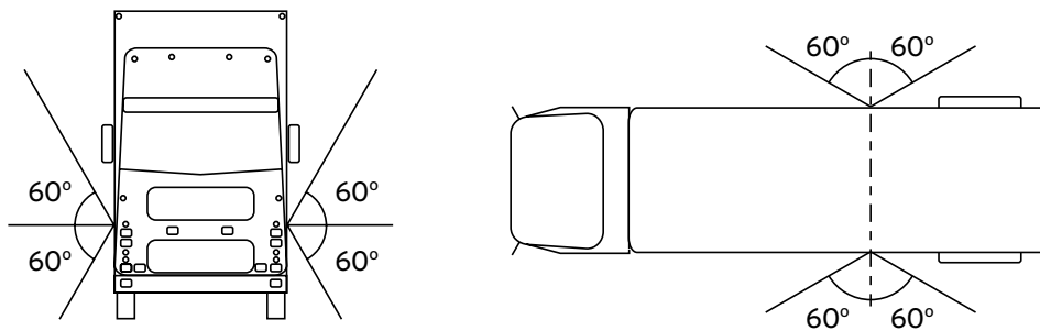
Figure 4-8-1. Visibility angles for side-marker lamps
