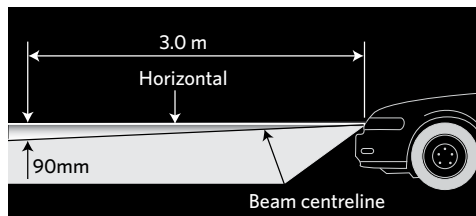
(b) Beam dip angle
