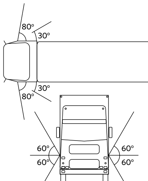
Figure 4-5-2. Required angles for side-facing direction indicator lamps
