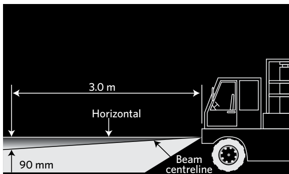
(b) Beam dip angle
