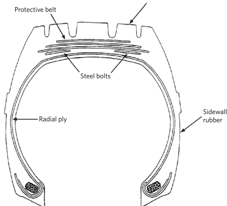
Figure 10-1-1. Cross-sectional representation of a heavy vehicle radial-ply tyre
