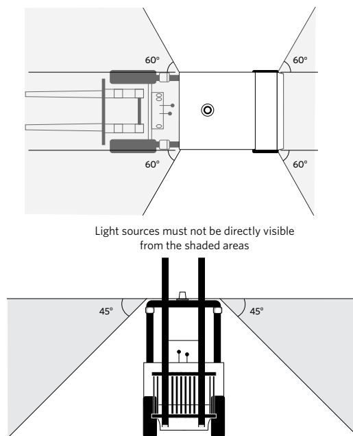
Figure 4-15-1. Visibility angles for cosmetic lamps
