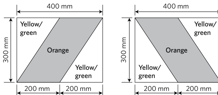
Figure 2-2-1. Hazard panel details
