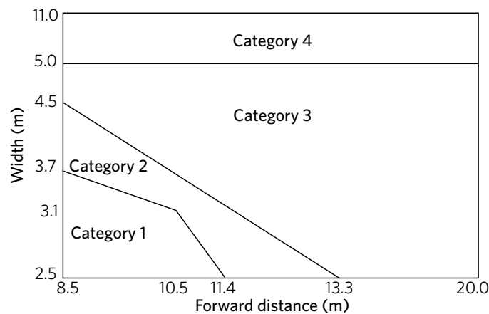
Figure 2-2-3. Overdimension vehicle categories for width/forward distance thresholds
