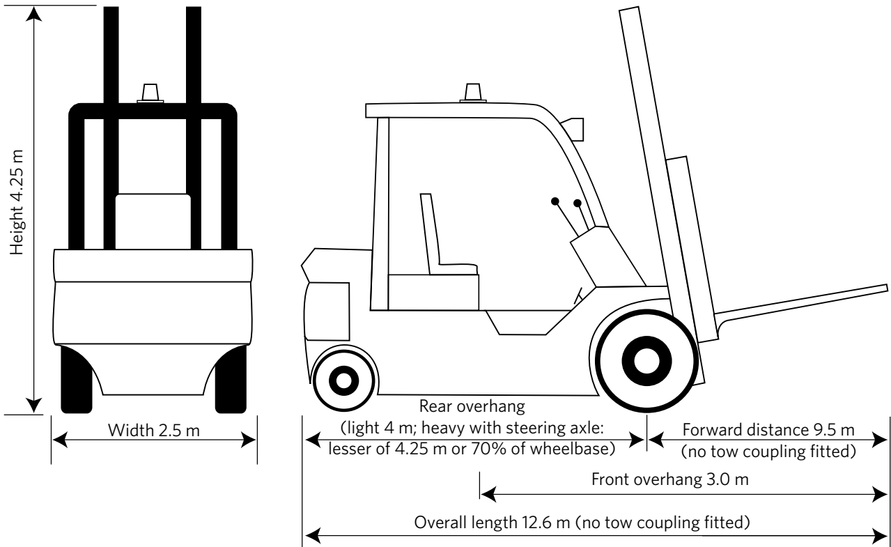
Figure 2-2-4. Dimension requirements
