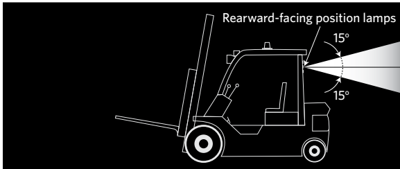
(a) Vertical beam angles
