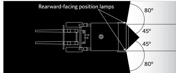
(b) Horizontal beam angles
