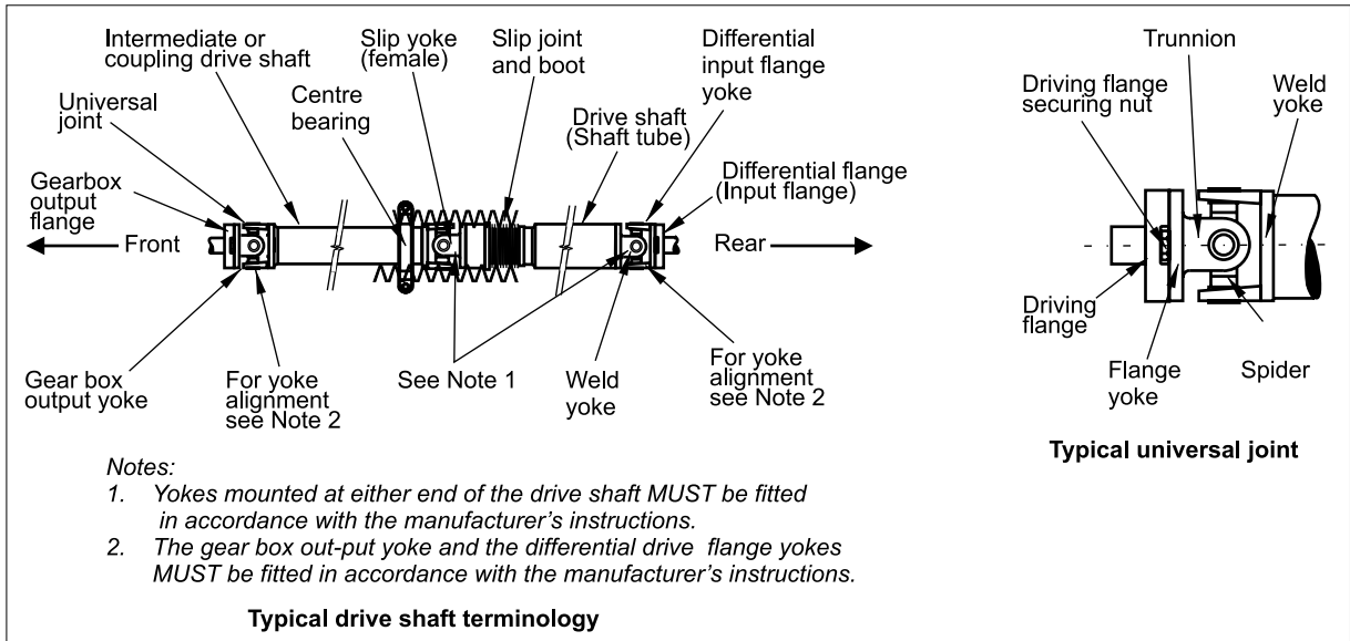
Figure 13-1-1. A typical driveshaft assembly
