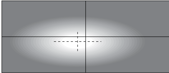
Figure 4-1-5. Symmetric dipped-beam headlamp pattern on light board
