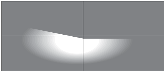
Figure 4-1-3. Asymmetric dipped-beam headlamp pattern on light board
