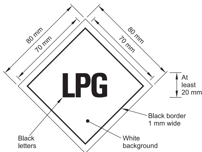
Figure 1-2-1. LPG vehicle identification label
