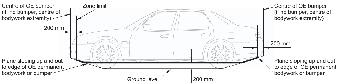
Figure 2-7-2. Ground clearance zone limits for a small vehicle (requirements from AS/NZS 2739: 2003)
