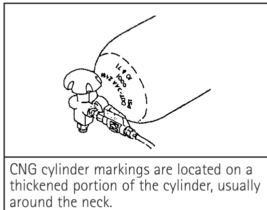
Figure 2-3-1. Cylinder markings
