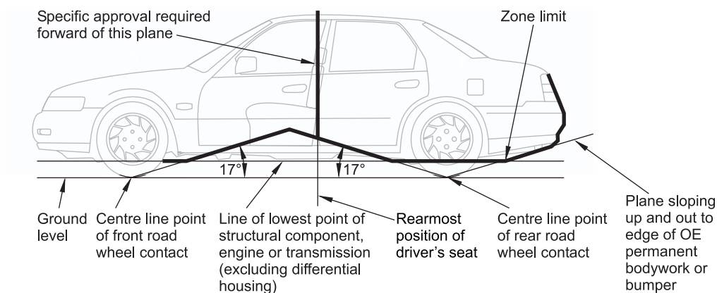
Figure 2-7-1. Zone limit for container location (requirements from NZS 5422: 1987: Part 2)
