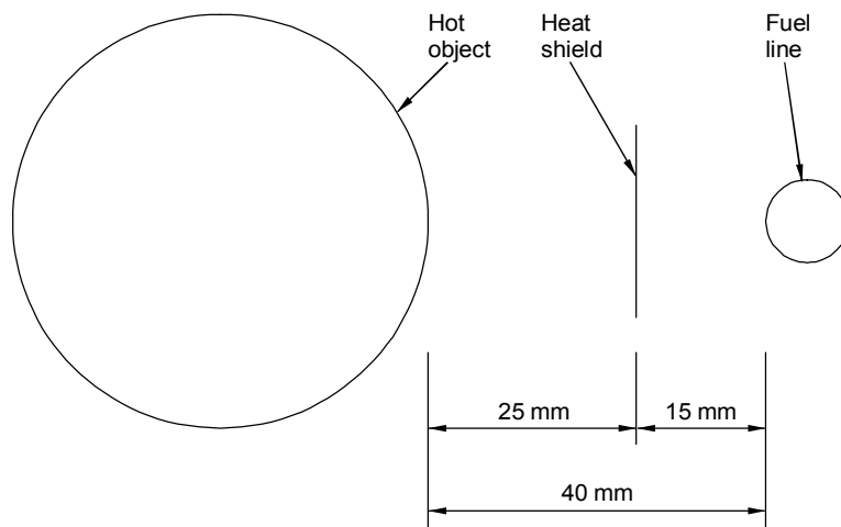
Figure 2-8-1. Minimum fuel line distance to hot object with heat shield
