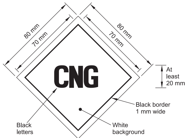
Figure 2-2-1. CNG vehicle identification label
