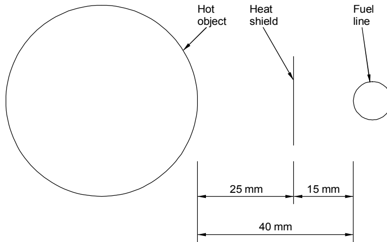
Figure 1-9-1. Minimum fuel line distance to hot object with heat shield
