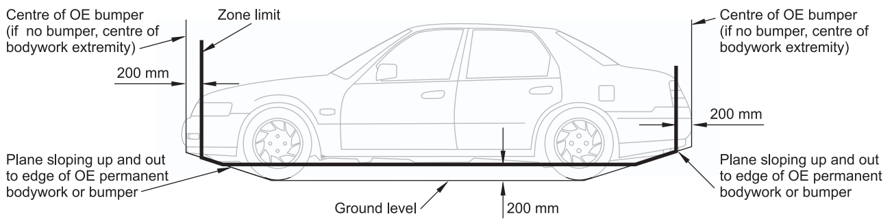
Figure 1–8–2. Ground clearance zone limits for a small vehicle (requirements from AS/NZS 1425:2003)
